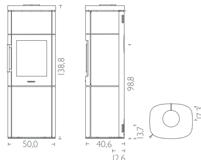
HWAM 4560m with soapstone cover
