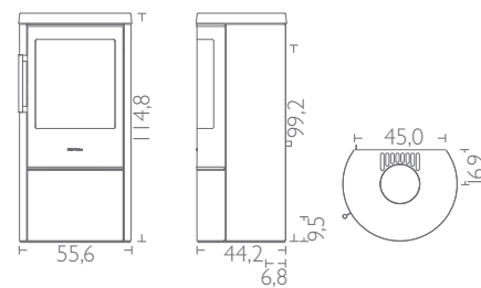
HWAM 3640m, white
