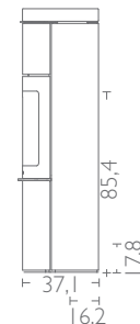
HWAM 3520c with grey sandstone cover
