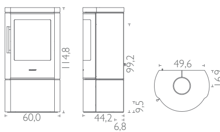
HWAM 3640c with soapstone cover
