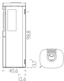
HWAM 4530c with side glasses
