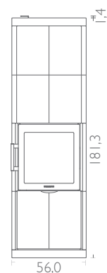
HWAM 7180c with soapstone cover
