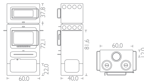
HWAM Classic 4 with plinth and baking oven
