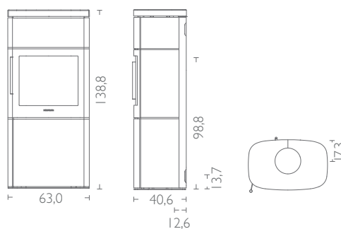
HWAM 4660m with Tobacco sandstone cover
