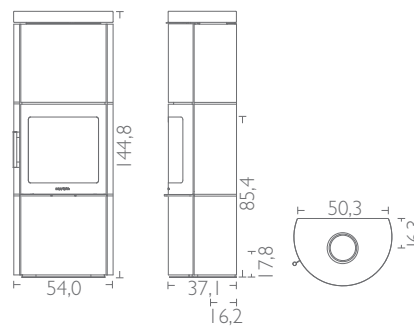
HWAM 3530c with soapstone cover
