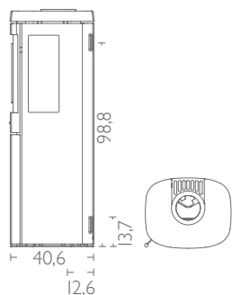
HWAM 4530m with side glasses
