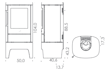
HWAM 4520m with high plinth
