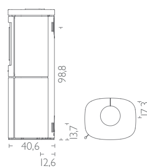
HWAM 4540c with soapstone cover
