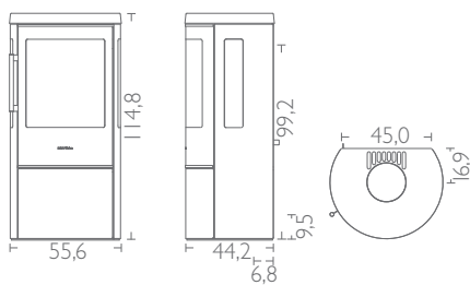
HWAM 3630c with side glasses
